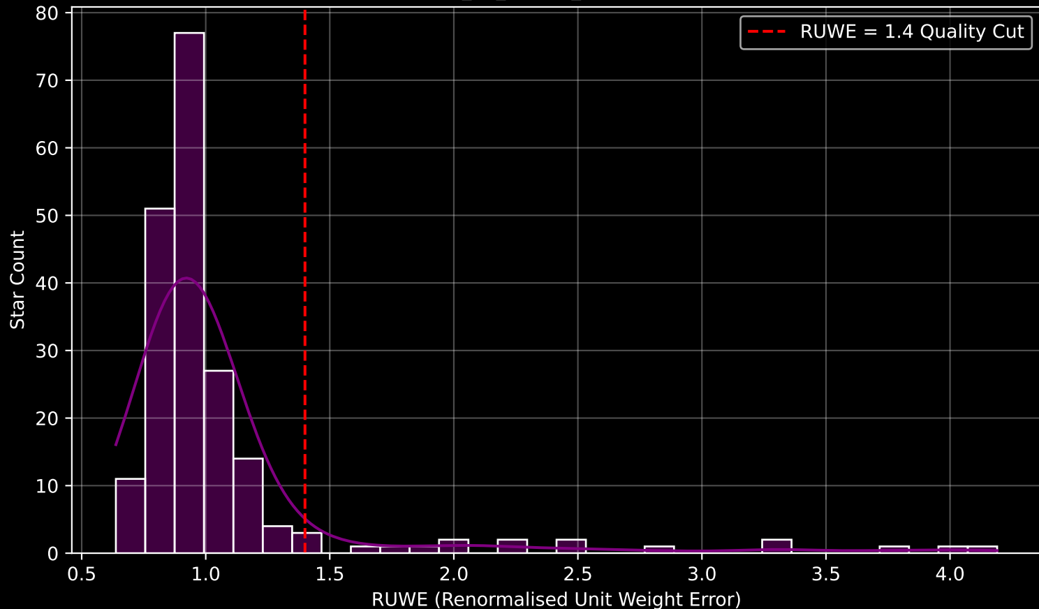
GAPOGEE DR17 Field [K2_C7_012-08_btx] RUWE Distribution (n= 202)
