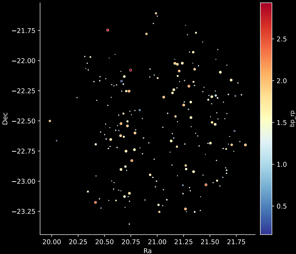
APOGEE DR17 Field: [K2_C7_012-08_btx] Stars: 208
