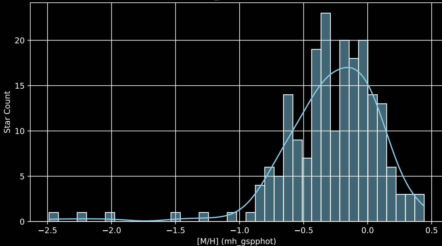
APOGEE DR17 Field: [K2_C7_012-08_btx [M/H] (mh_gspphot) (n= 204)
