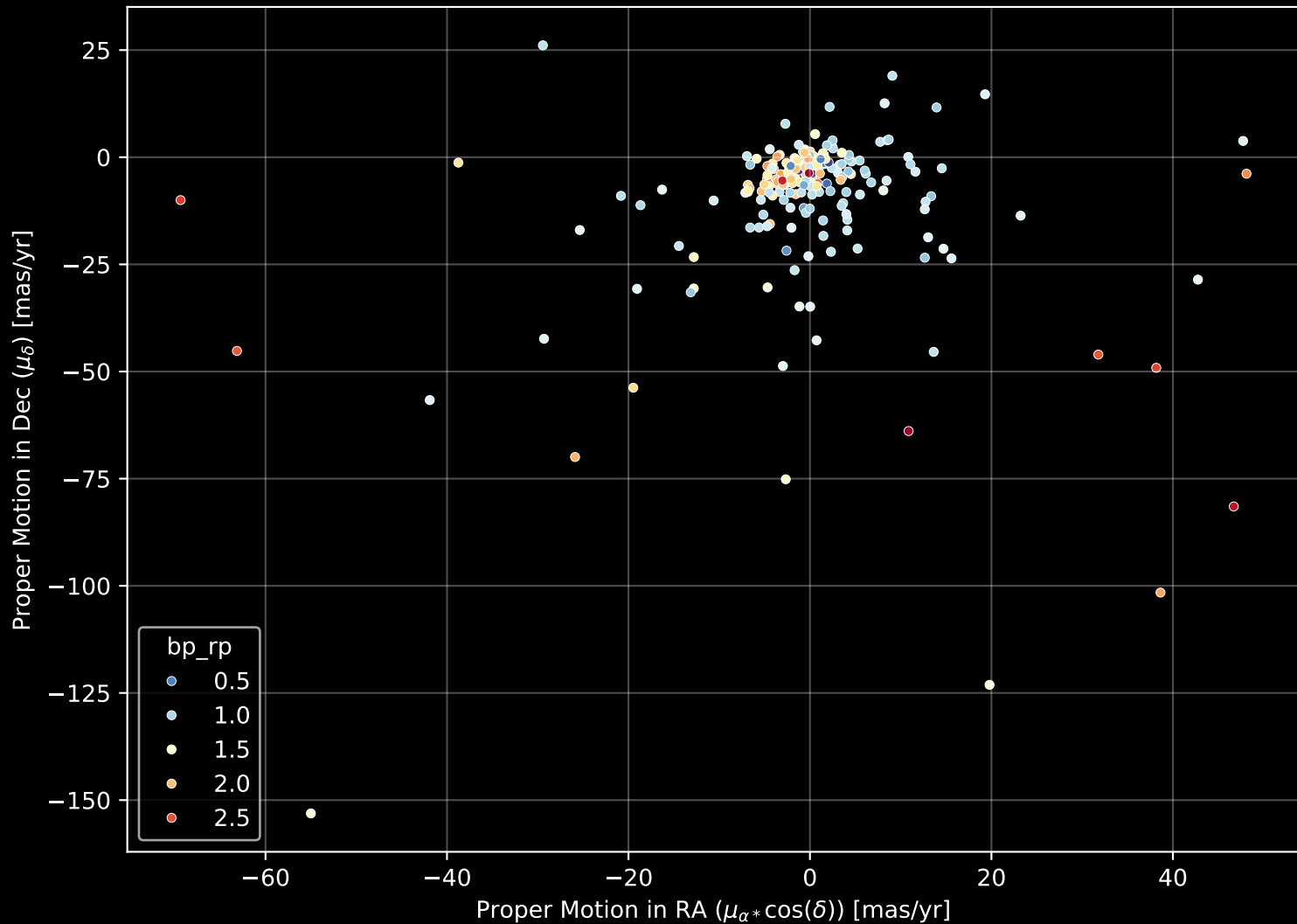
APOGEE DR17 Field: [K2_C7_012-08_btx] Proper Motion Diagram (n= 208)
