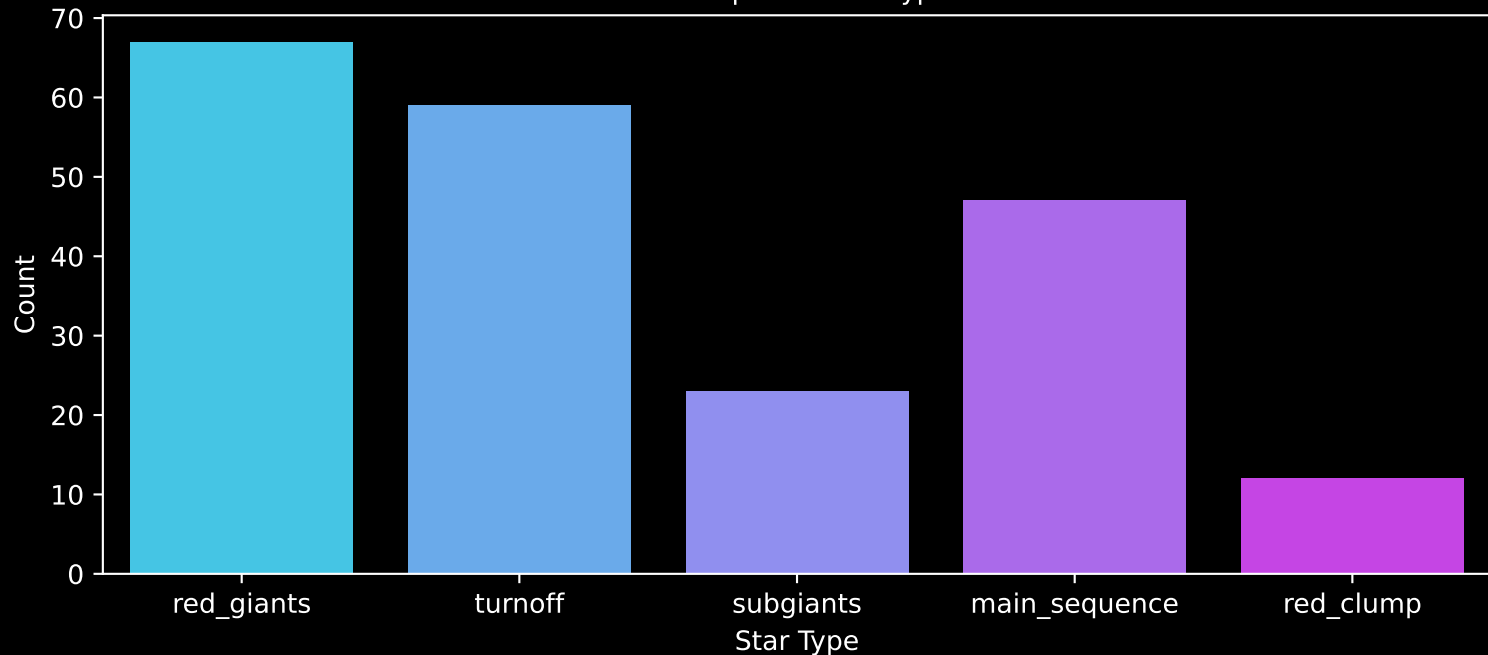
APOGEE DR17 Field: [K2_C7_012-08_btx] Count plot of Star Type
