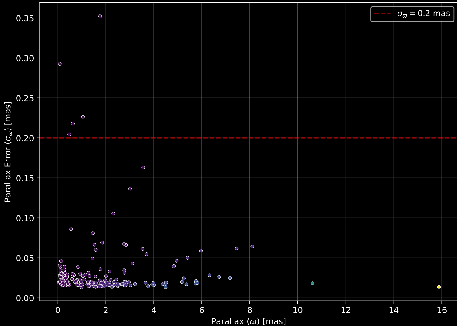
APOGEE DR17 Field: [K2_C7_012-08_btx] Parallax Quality (n= 208)
